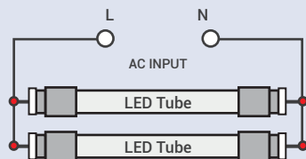
Double-ended input
